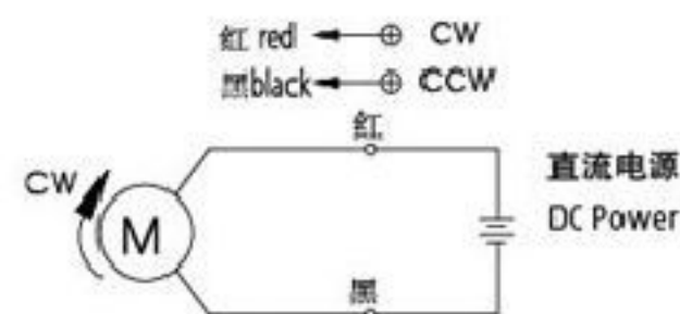
电机接线图Wiring Diagram of Motor
