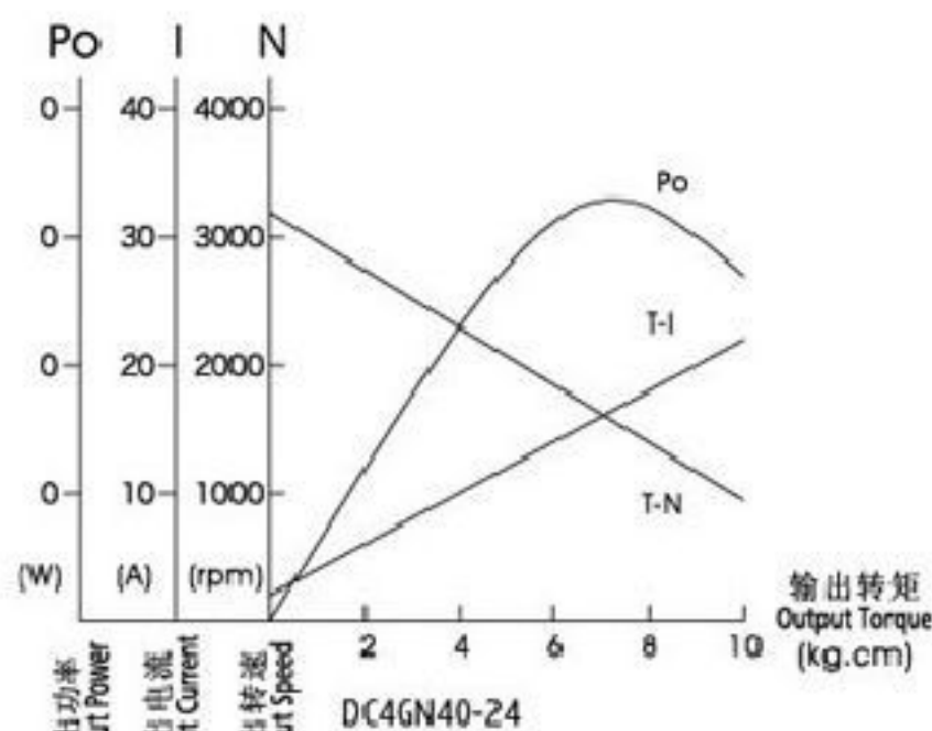
电机特性曲线 Characteristic Curve of Motor
